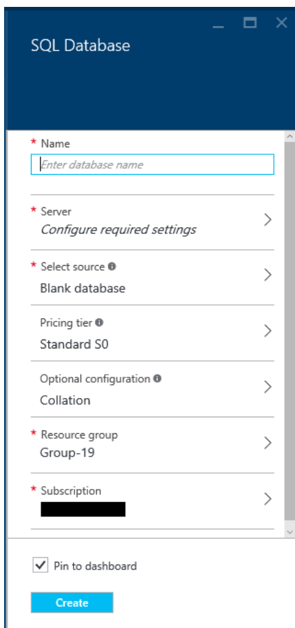
Figure 3-10: Creating a new database
