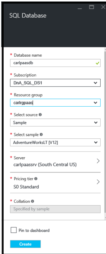
Figure 3-20: Completed SQL Database blade
