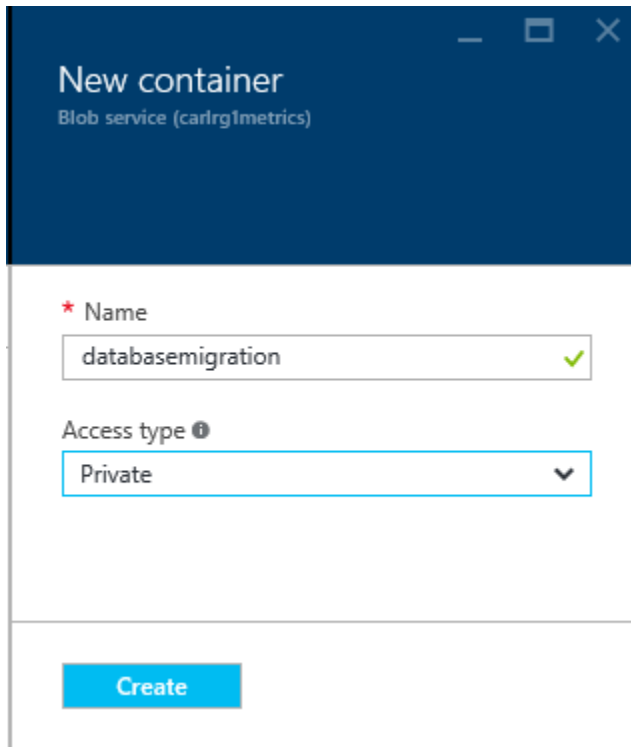
Figure 4-12: New container creation
