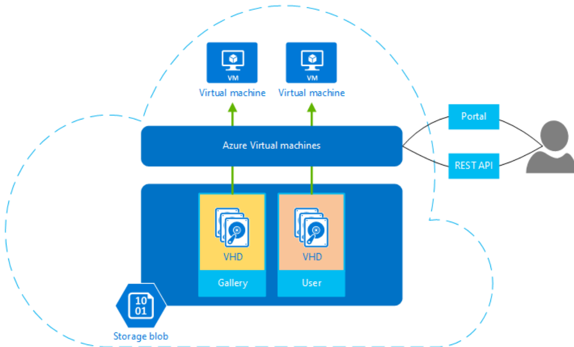
Figure 1-3: Azure virtual machines (Azure VMs)
