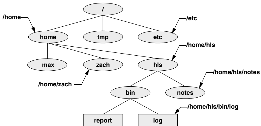
Figure 4-5 Absolute pathnames
