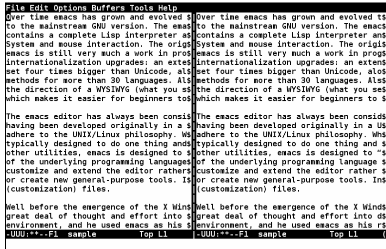
Figure 7-10 Splitting a window horizontally
