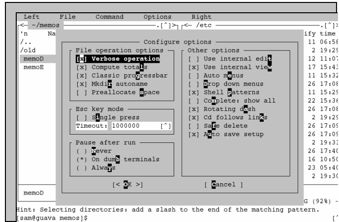
Figure VI-5 The Configure options window
