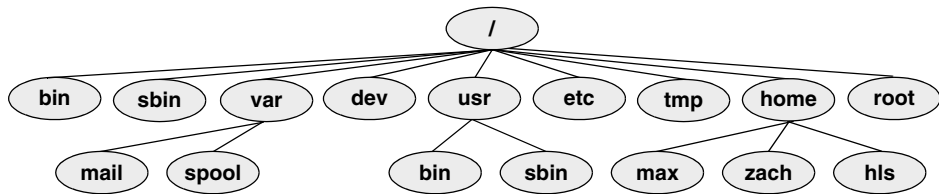
Figure 4-11 A typical FHS-based Linux filesystem structure
