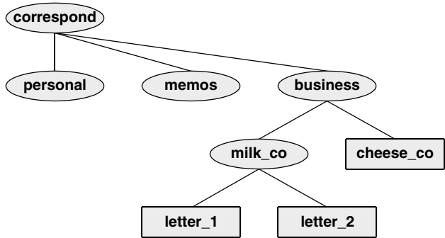
Figure 4-2 A secretary’s directories
