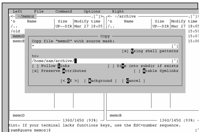
Figure VI-6 The Copy window
