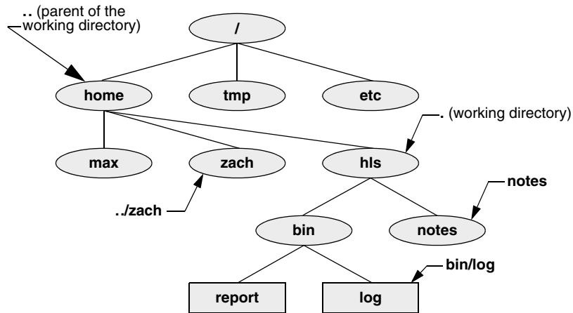
Figure 4-6 Relative pathnames
