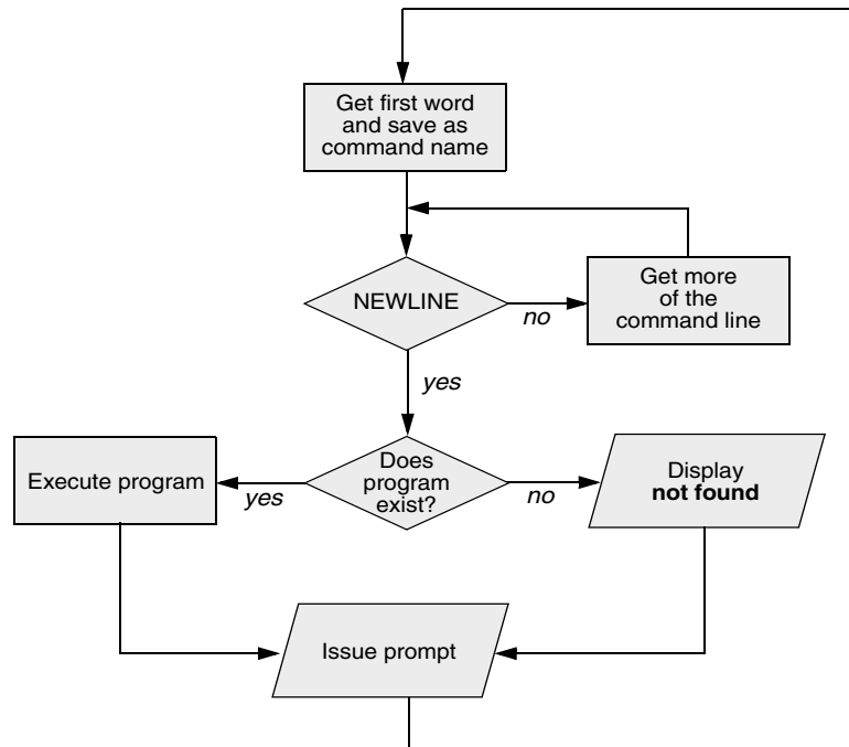
Figure 5-2 Processing the command line
