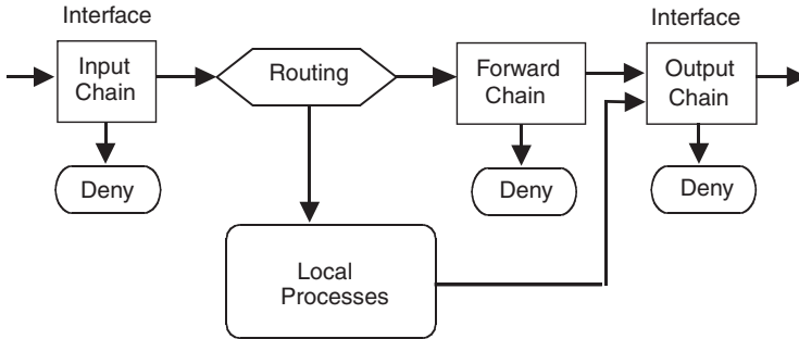
Figure 3.1 IPFW packet traversal
