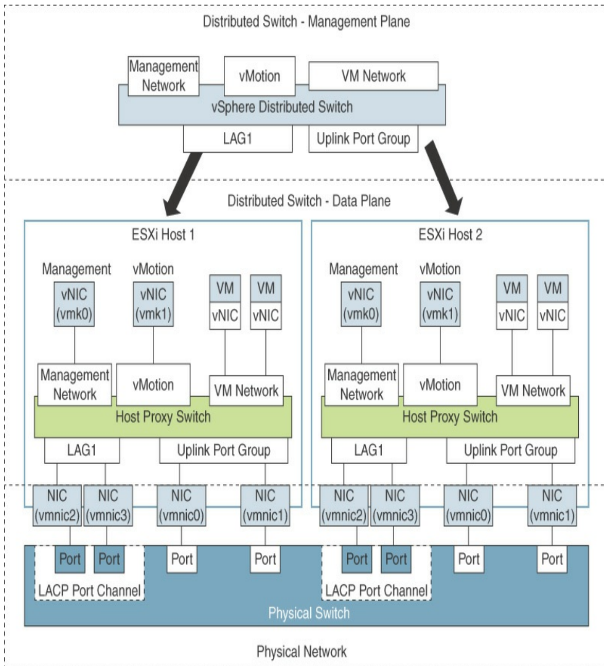
FIGURE 3-4 LACP Configuration with a vDS
