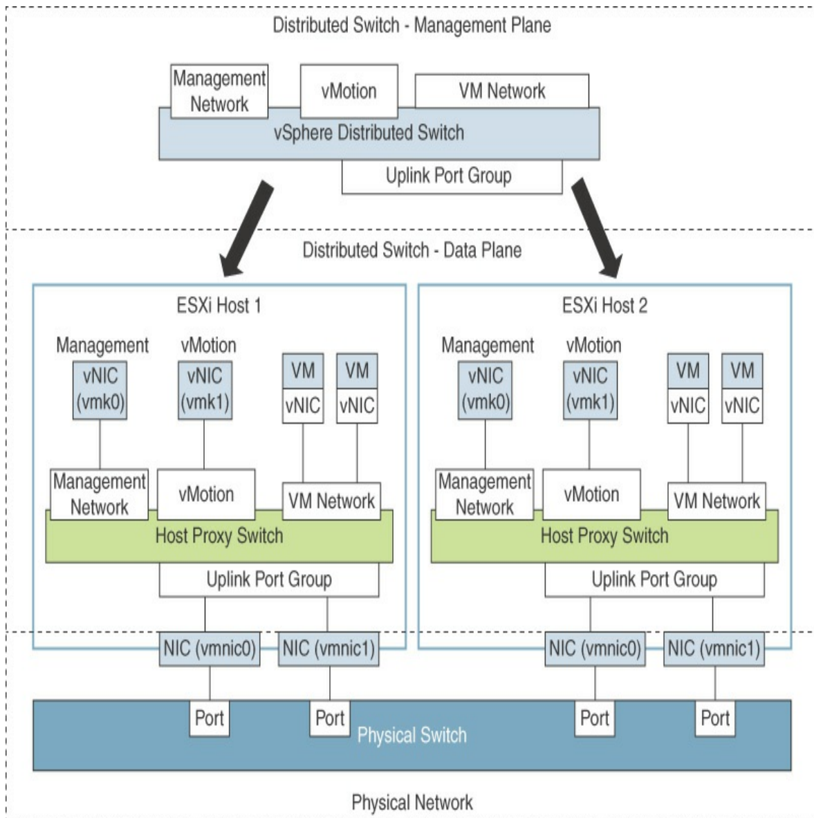
FIGURE 3-2 vDS Architecture
