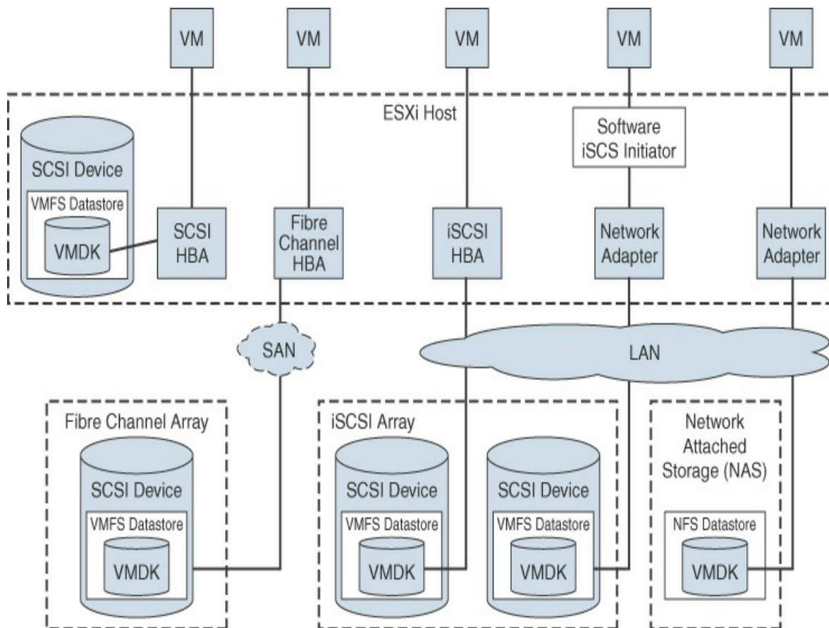
FIGURE 2-1 Virtual Machine Storage
