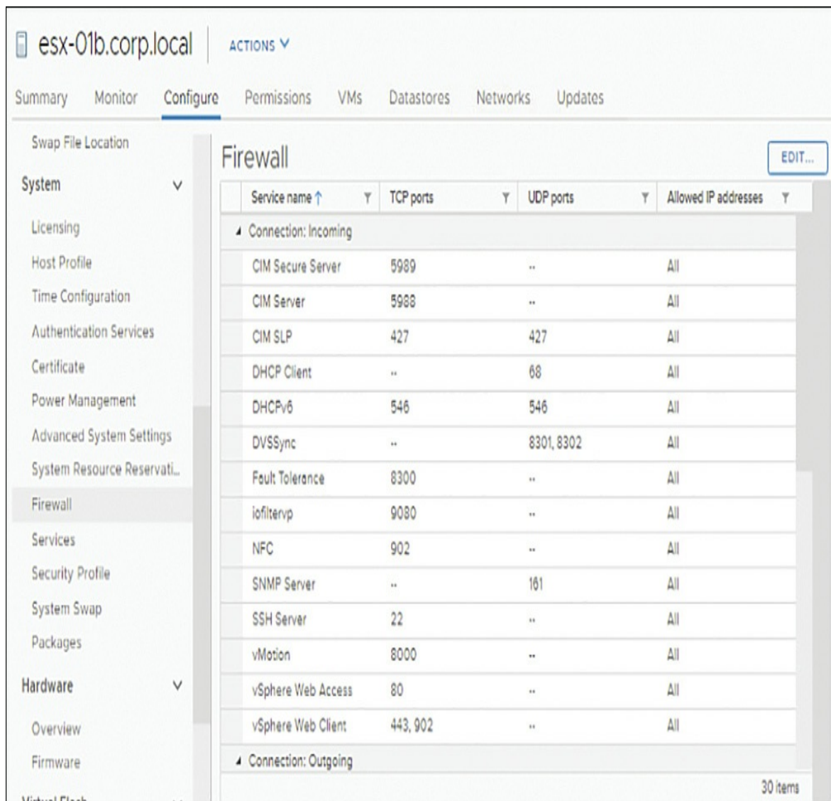
FIGURE 13-2 Firewall Rules in the vSphere Client
