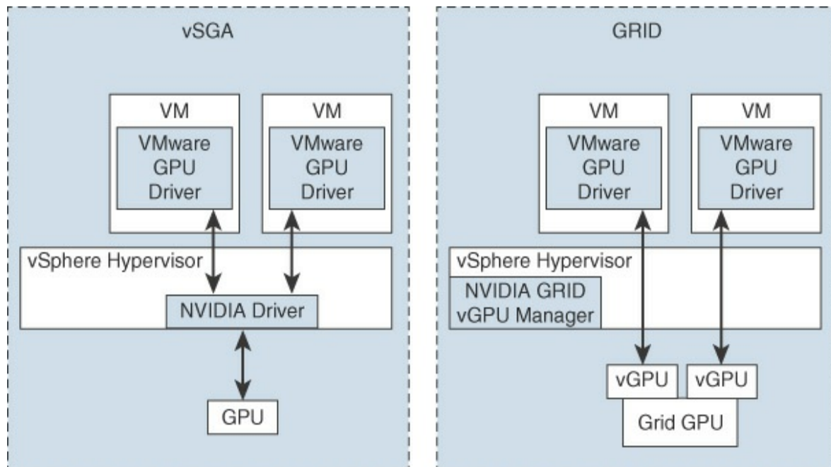
FIGURE 14-1 Comparison of the vSGA and GRID Models
