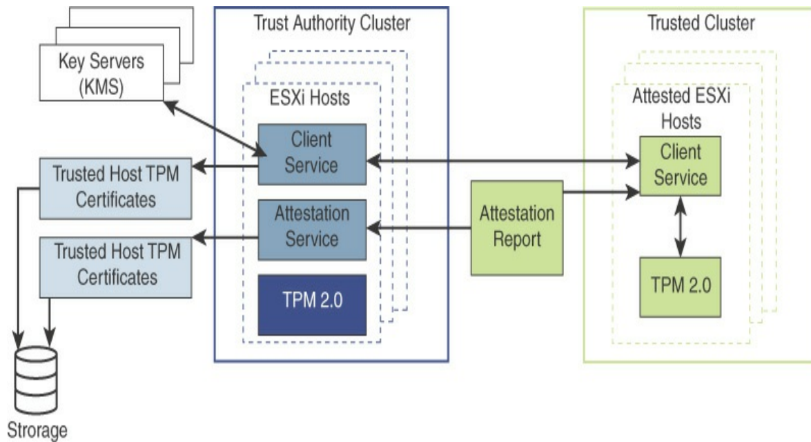
FIGURE 7-5 vSphere Trusted Authority Architecture
