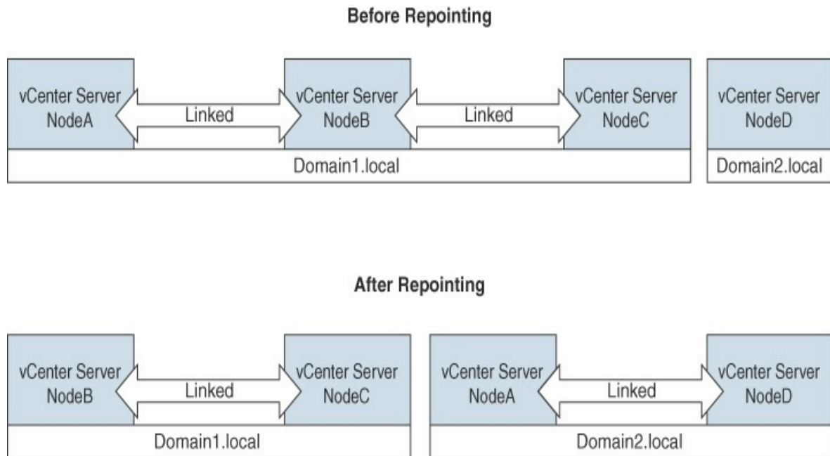
FIGURE 13-4 Repointing vCenter from a Multi-Node Domain
