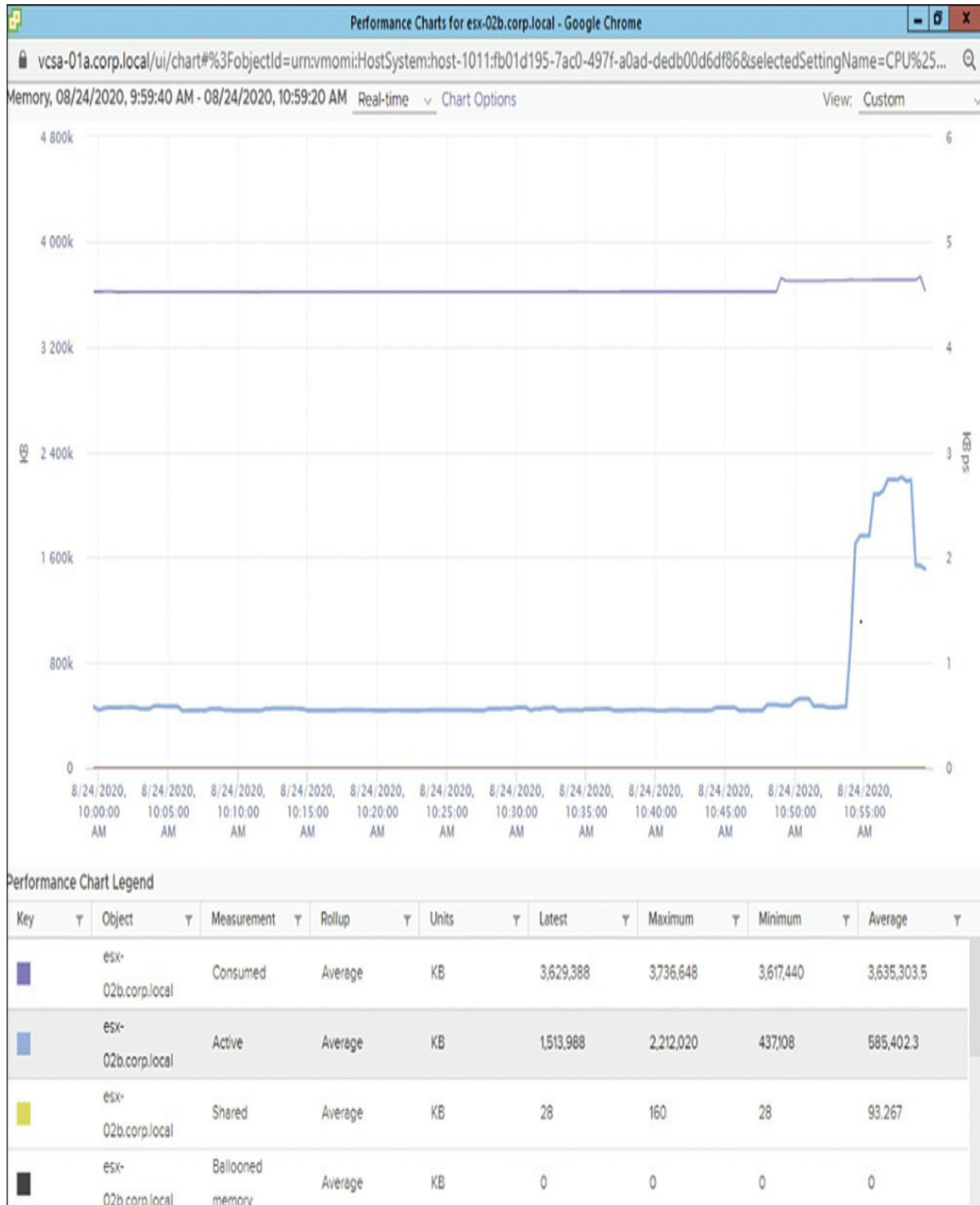
FIGURE 10-1 Sample Advanced Performance Chart
