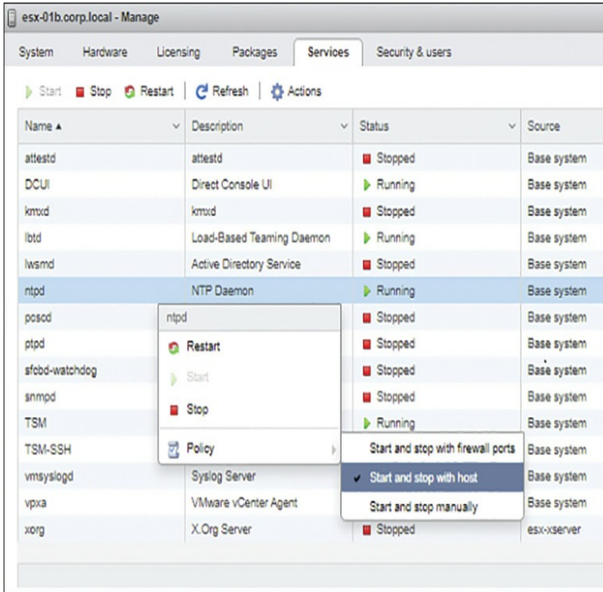
FIGURE 13-1 Managing Host Services in the vSphere Host Client
