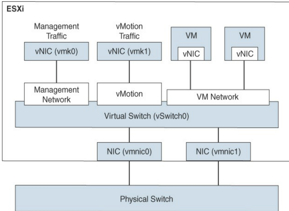
FIGURE 3-1 A Sample Virtual Switch
