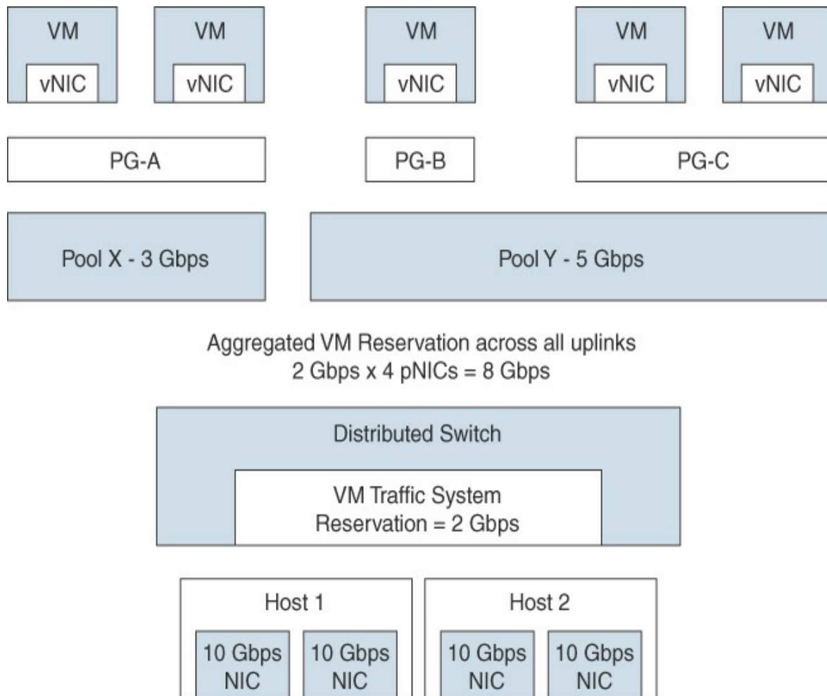
FIGURE 3-3 Network Resource Pools Example
