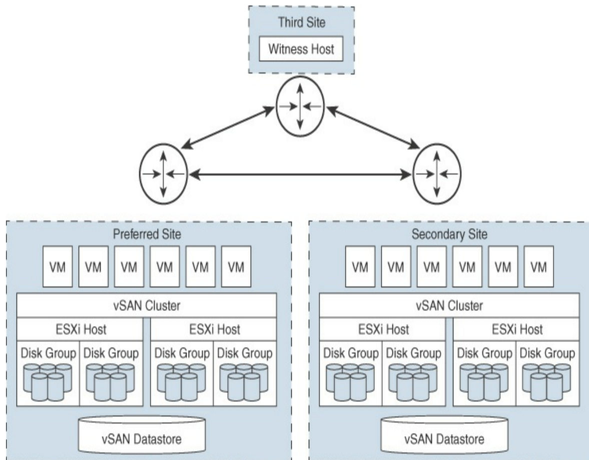
FIGURE 2-5 A Stretched vSAN Cluster
