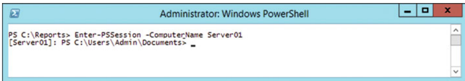
Figure 8-2. Enter-PSSession
