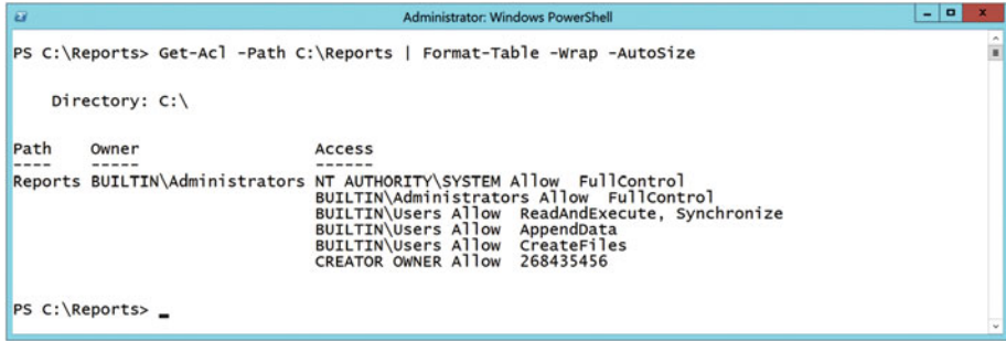
Figure 3-8. Get-Acl
